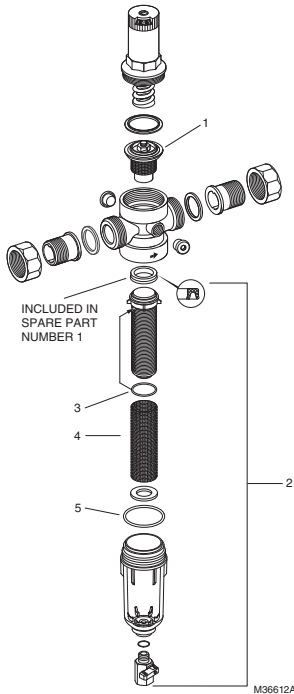
Fig. 5. Spare parts diagram.
