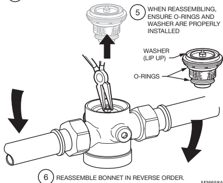
Fig. 4. Replacing the FK06 cartridge.
