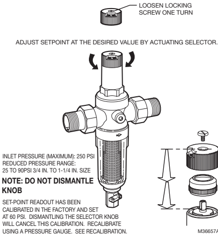
Fig. 2. Changing outlet pressure.
