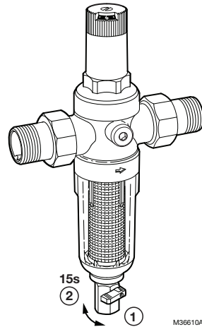
Fig. 3. Rinsing the filter.
