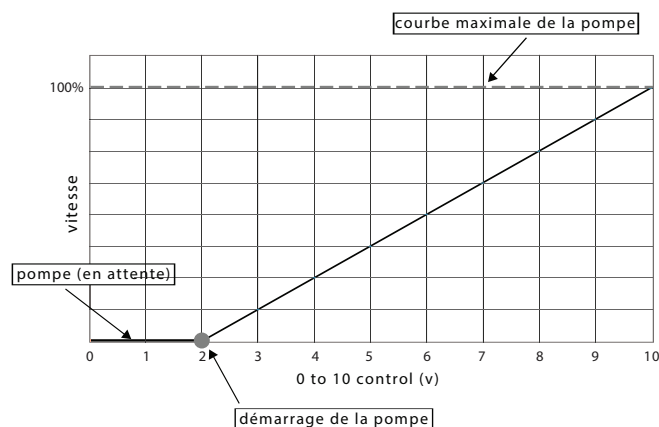
Fig. 6. 0-10 V operation
