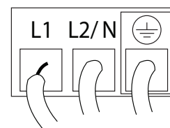
Fig. 4. Power supply connection
