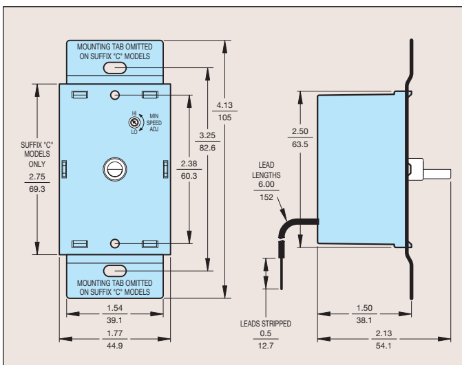
KBWC-15, 16, 25, 26, 35, 36 (Pkg. C) Mechanical Specifications (Inches/mm)
