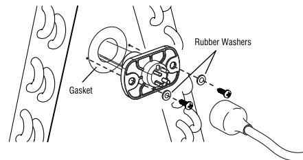
Fig. 5. Insert lamp into delta plate knockout and secure with screws and washers. Connect remote lamp extension cord.
