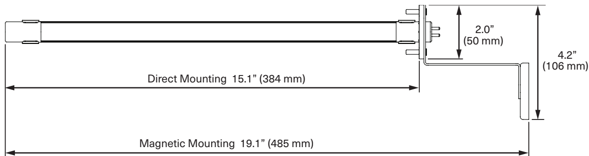
Fig. 2. Minimum clearances.
