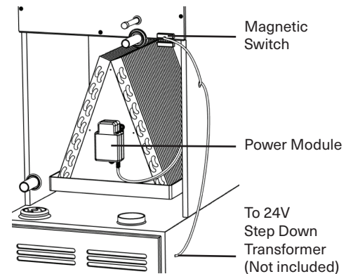
Fig. 9. Connect magnetic switch and power cord.
