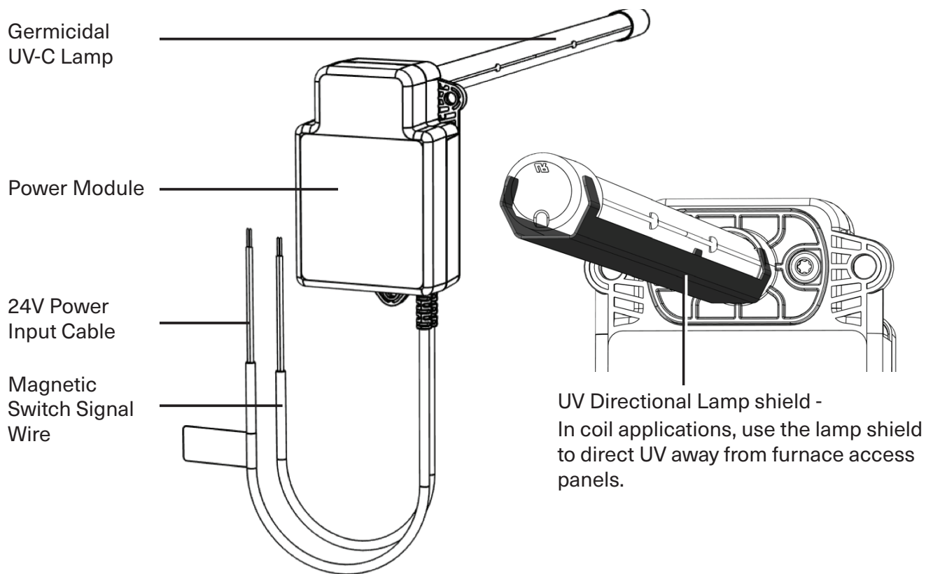
Fig. 1. Unit component identification.
