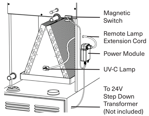
Fig. 6. Secure power module to air handler or duct with long screws. Do not overtighten.
